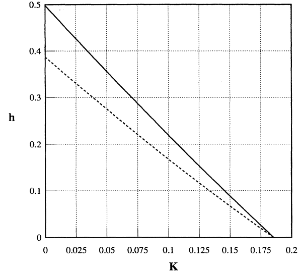
FIG. 2. Phase diagram in the K - h plane: the solid and dashed lines correspond to Hamiltonians \mathcal{H} and \mathcal{H}_{\text{alt}} , respectively.
