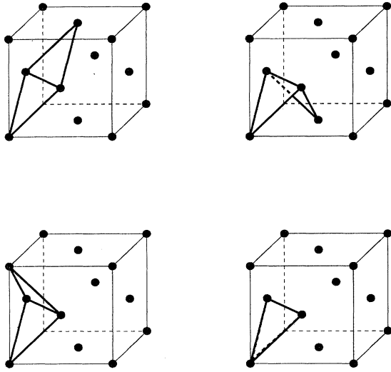
FIG. 1. The four possible foldings of two adjacent plaquettes of the triangular lattice embedded in a fcc lattice are shown. From the left to the right and from the top to the bottom: no fold, acute fold ( 70^\circ 32' ), obtuse fold ( 109^\circ 28' ), and complete fold. The dots represent the vertices in an elementary cell of the fcc lattice.
